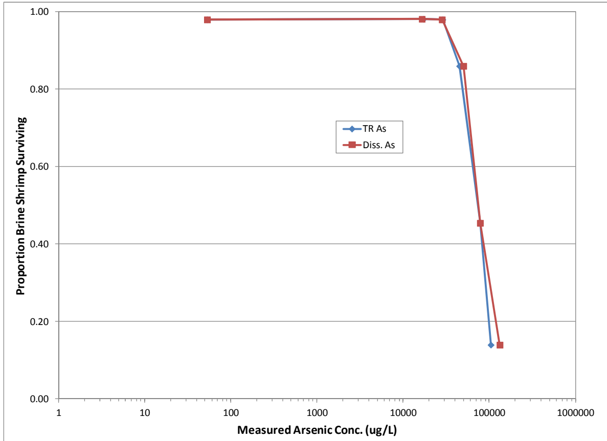
Figure 1. Proportion of Artemia franciscana Surviving at 96 hours versus Measured Arsenic Concentrations.
